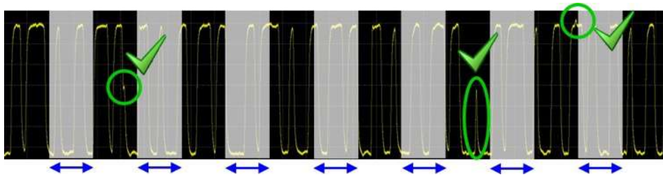
Figure 5. InfiniiVision 4000 X-Series with 1,000,000 waveforms/second. A short dead time (gray areas) increases your chances of capturing infrequent events.
