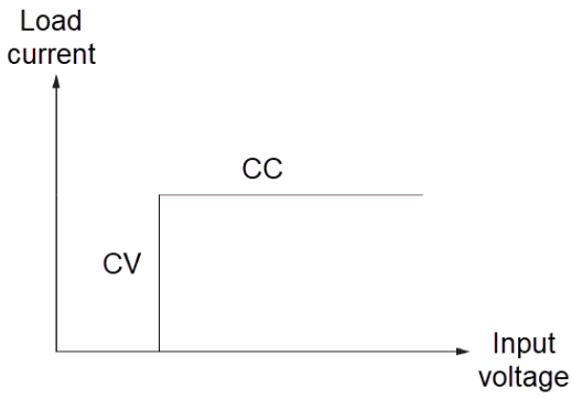
CV+CC mode
